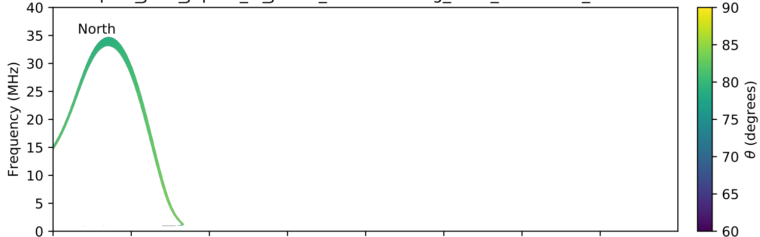
expres_juno_jupiter_io_jrm09_lossc-wid1deg_3kev_20190315_v01.cdf
