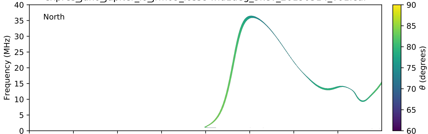
expres_juno_jupiter_io_jrm09_lossc-wid1deg_3kev_20190314_v01.cdf
