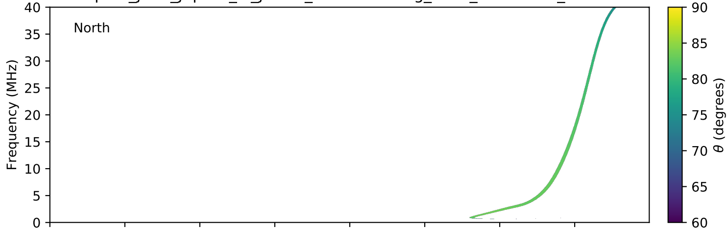
expres_juno_jupiter_io_jrm09_lossc-wid1deg_3kev_20190312_v01.cdf
