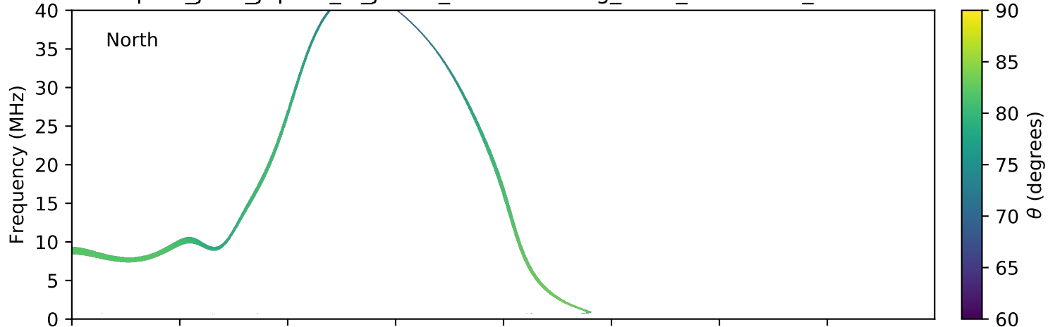
expres_juno_jupiter_io_jrm09_lossc-wid1deg_3kev_20190311_v01.cdf
