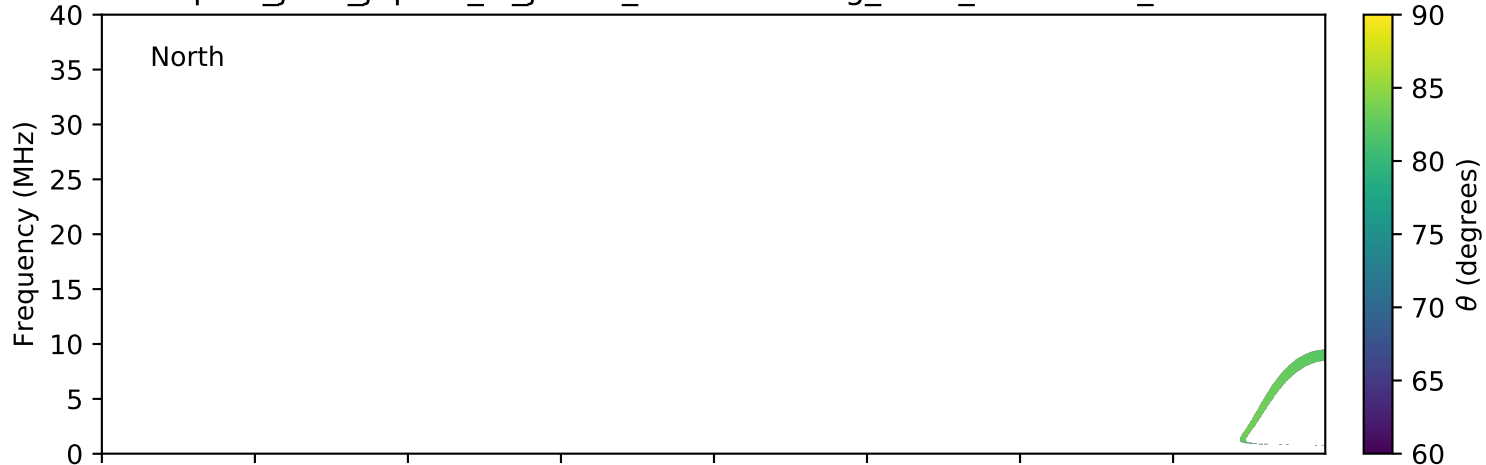
expres_juno_jupiter_io_jrm09_lossc-wid1deg_3kev_20190310_v01.cdf
