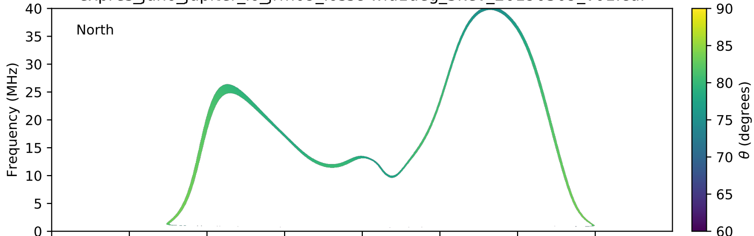
expres_juno_jupiter_io_jrm09_lossc-wid1deg_3kev_20190309_v01.cdf
