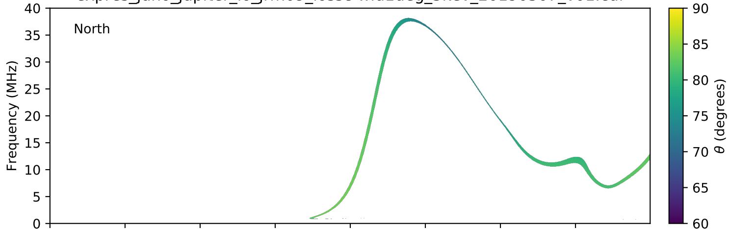
expres_juno_jupiter_io_jrm09_lossc-wid1deg_3kev_20190307_v01.cdf
