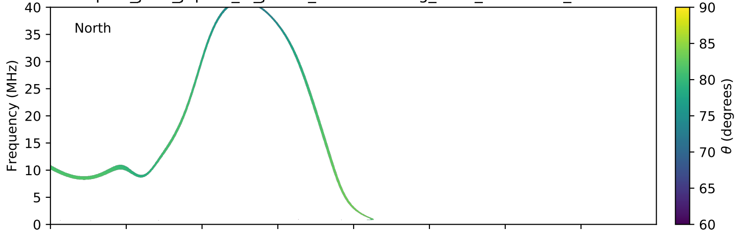
expres_juno_jupiter_io_jrm09_lossc-wid1deg_3kev_20190304_v01.cdf
