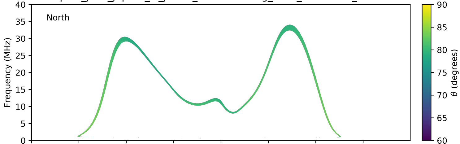
expres_juno_jupiter_io_jrm09_lossc-wid1deg_3kev_20190302_v01.cdf
