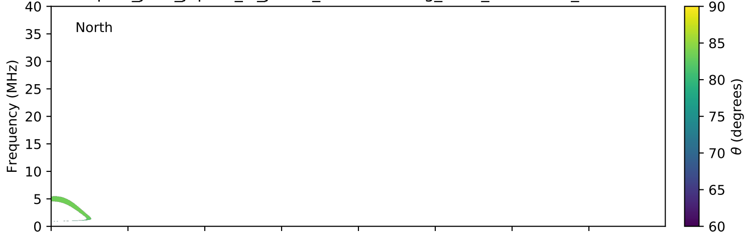
expres_juno_jupiter_io_jrm09_lossc-wid1deg_3kev_20190301_v01.cdf
