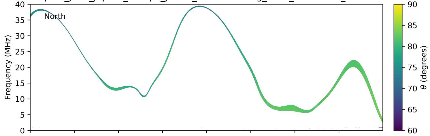
expres_juno_jupiter_europa_jrm09_lossc-wid1deg_3kev_20190327_v01.cdf
