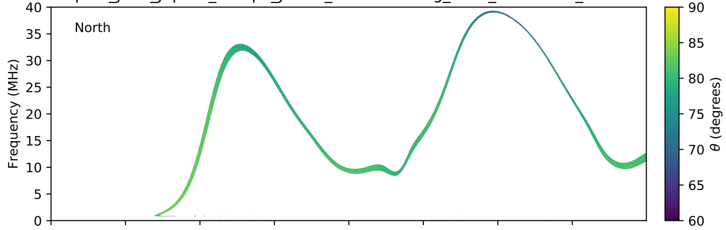
expres_juno_jupiter_europa_jrm09_lossc-wid1deg_3kev_20190323_v01.cdf
