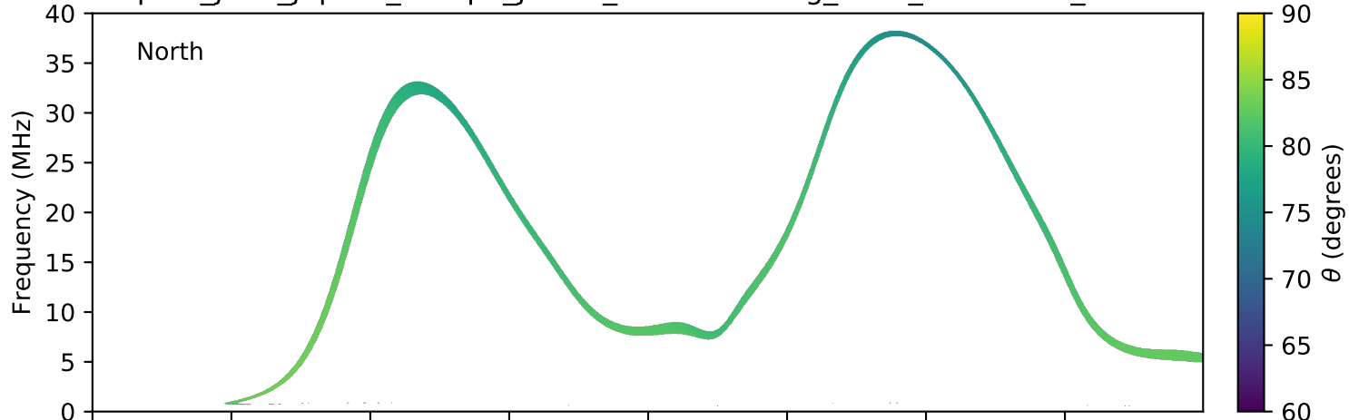
expres_juno_jupiter_europa_jrm09_lossc-wid1deg_3kev_20190316_v01.cdf
