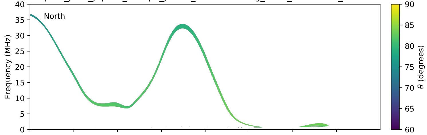
expres_juno_jupiter_europa_jrm09_lossc-wid1deg_3kev_20190313_v01.cdf
