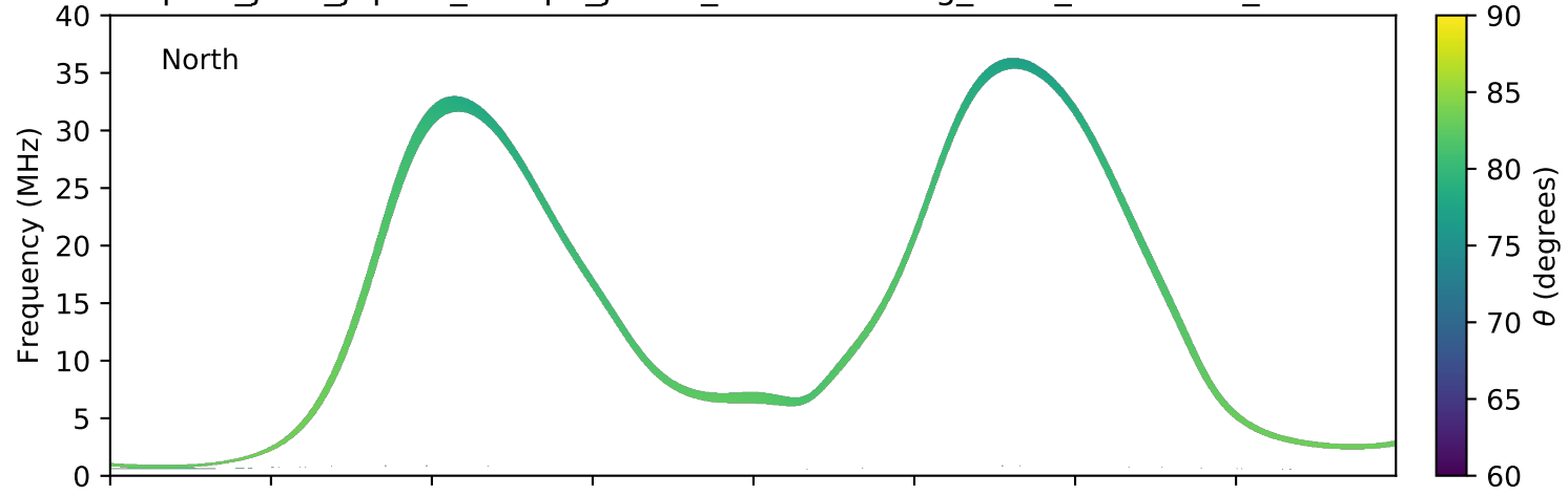
expres_juno_jupiter_europa_jrm09_lossc-wid1deg_3kev_20190309_v01.cdf
