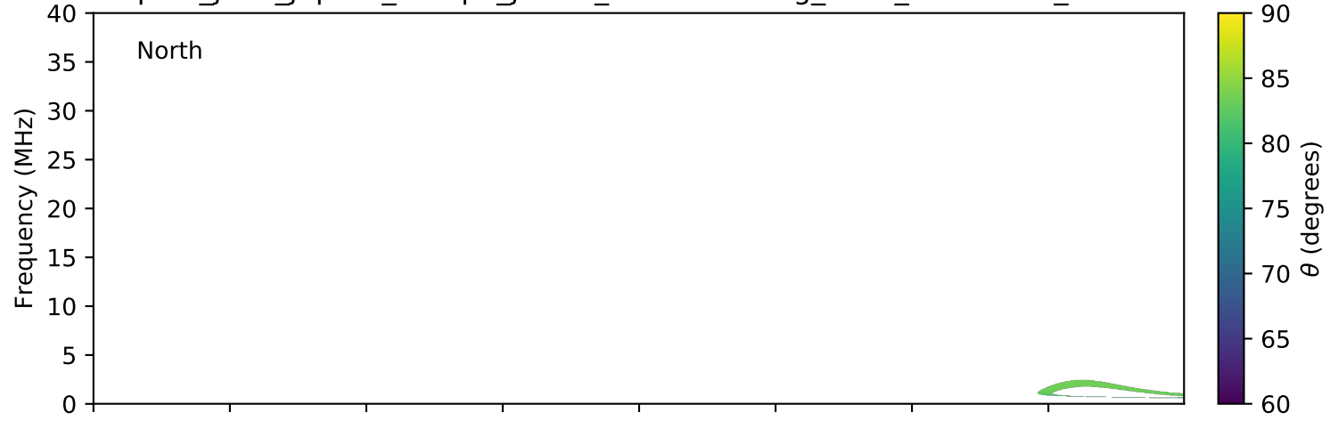
expres_juno_jupiter_europa_jrm09_lossc-wid1deg_3kev_20190308_v01.cdf
