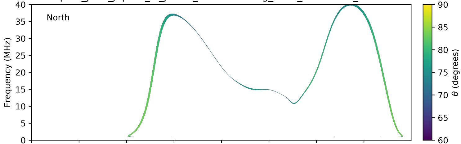
expres_juno_jupiter_io_jrm09_lossc-wid1deg_3kev_20190129_v01.cdf
