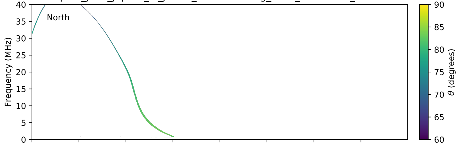
expres_juno_jupiter_io_jrm09_lossc-wid1deg_3kev_20190126_v01.cdf
