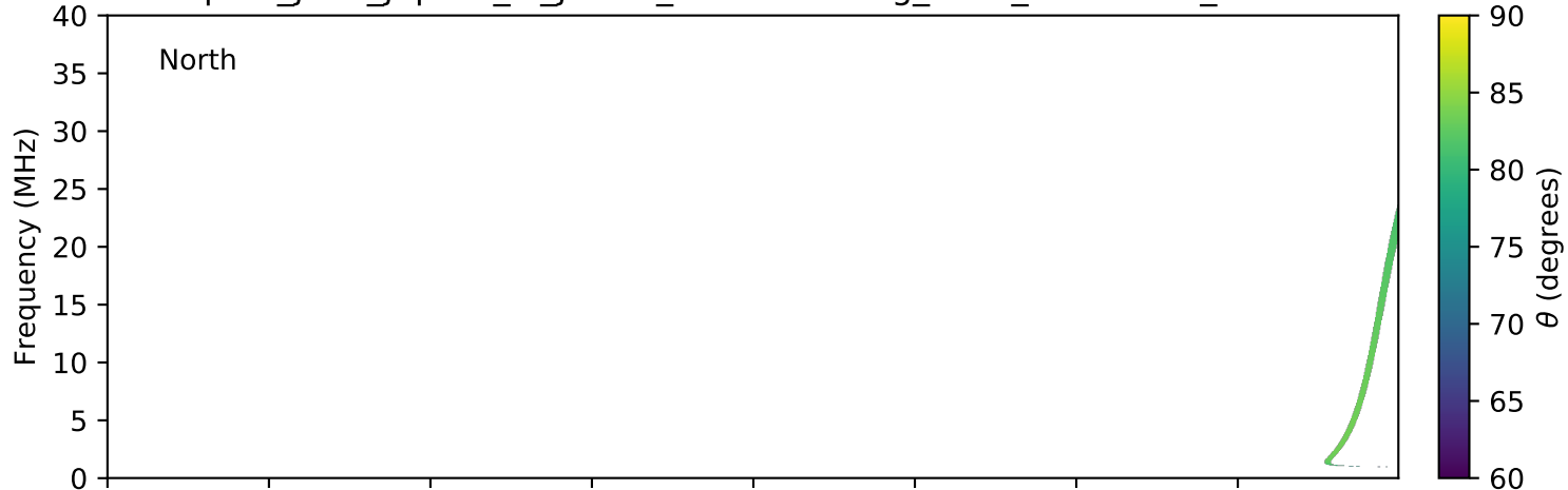
expres_juno_jupiter_io_jrm09_lossc-wid1deg_3kev_20190123_v01.cdf
