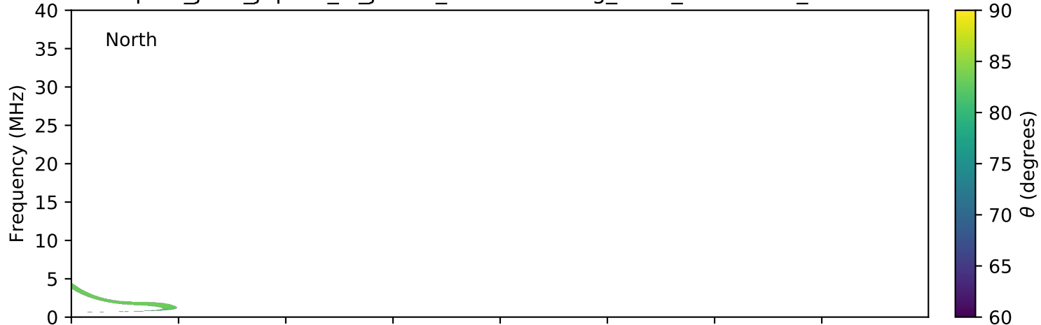
expres_juno_jupiter_io_jrm09_lossc-wid1deg_3kev_20190121_v01.cdf
