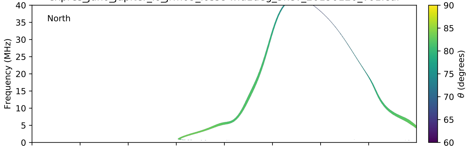
expres_juno_jupiter_io_jrm09_lossc-wid1deg_3kev_20190120_v01.cdf
