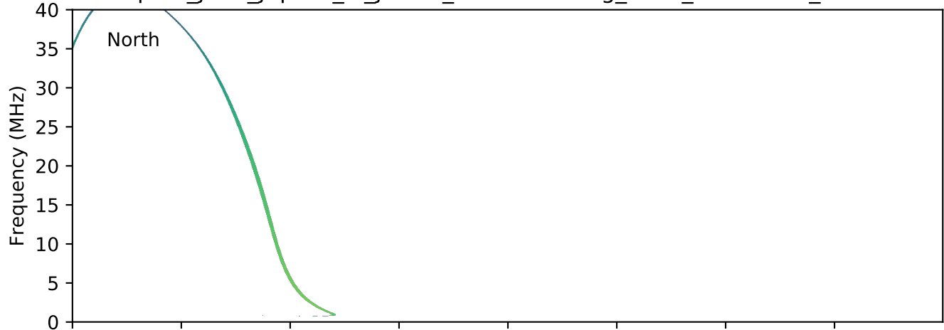
expres_juno_jupiter_io_jrm09_lossc-wid1deg_3kev_20190119_v01.cdf
