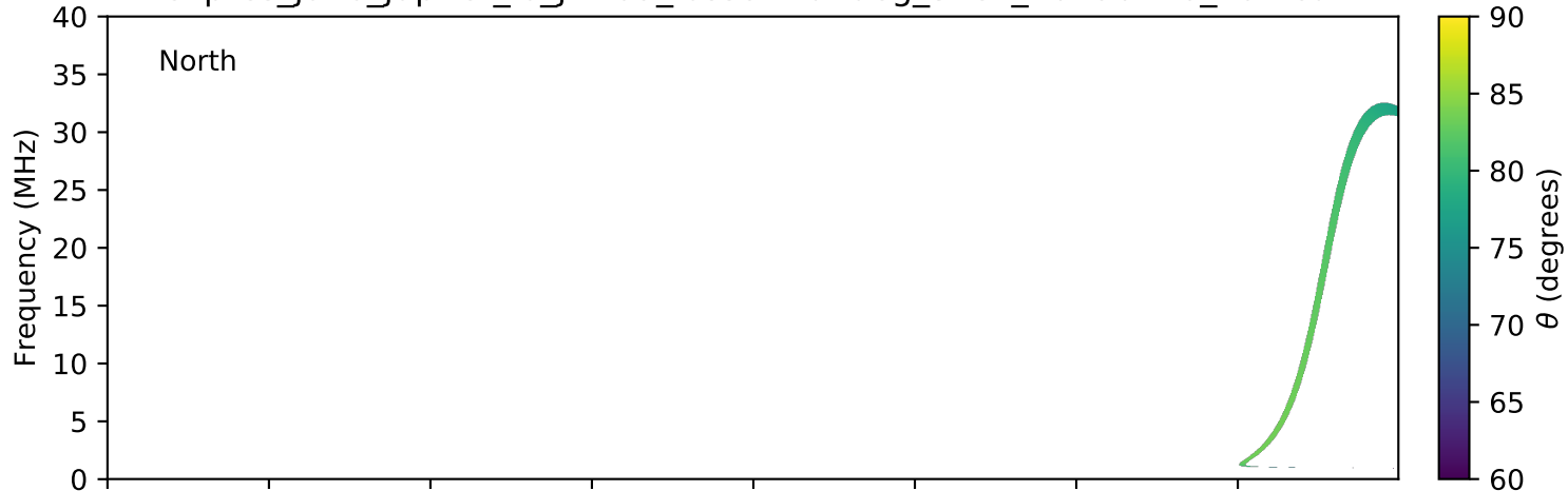
expres_juno_jupiter_io_jrm09_lossc-wid1deg_3kev_20190116_v01.cdf
