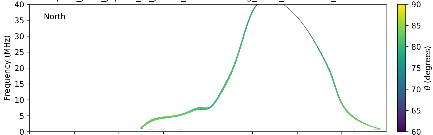
expres_juno_jupiter_io_jrm09_lossc-wid1deg_3kev_20190113_v01.cdf
