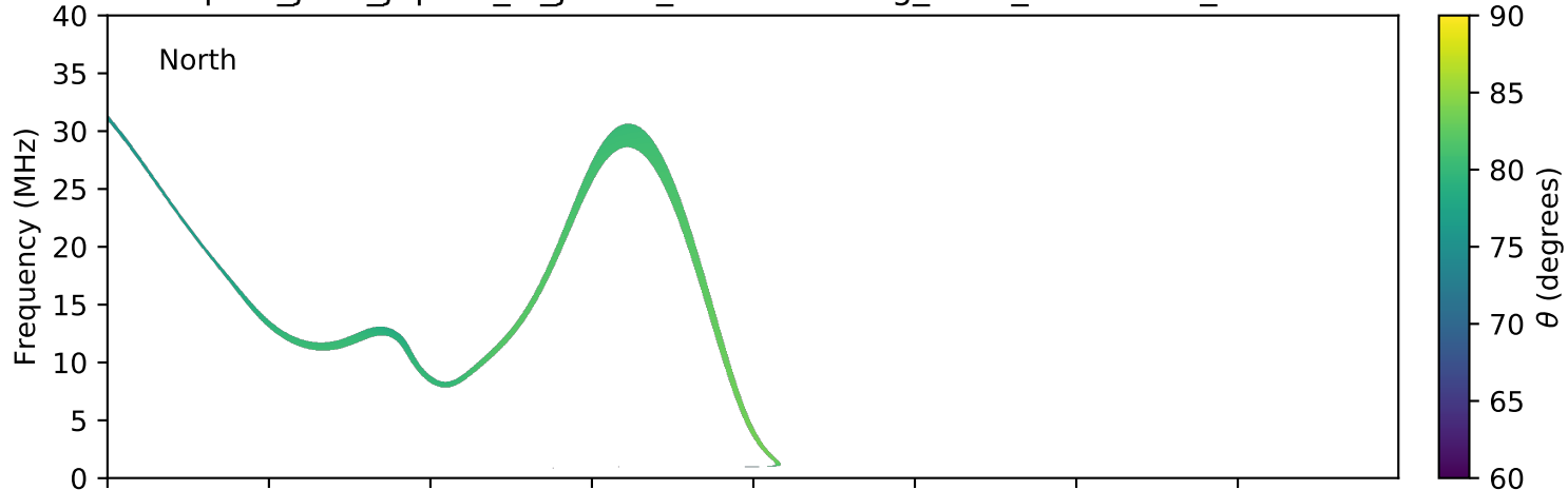
expres_juno_jupiter_io_jrm09_lossc-wid1deg_3kev_20190110_v01.cdf
