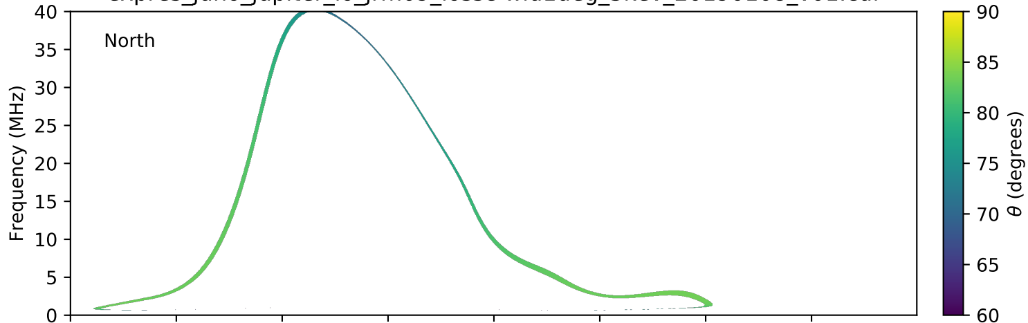
expres_juno_jupiter_io_jrm09_lossc-wid1deg_3kev_20190108_v01.cdf
