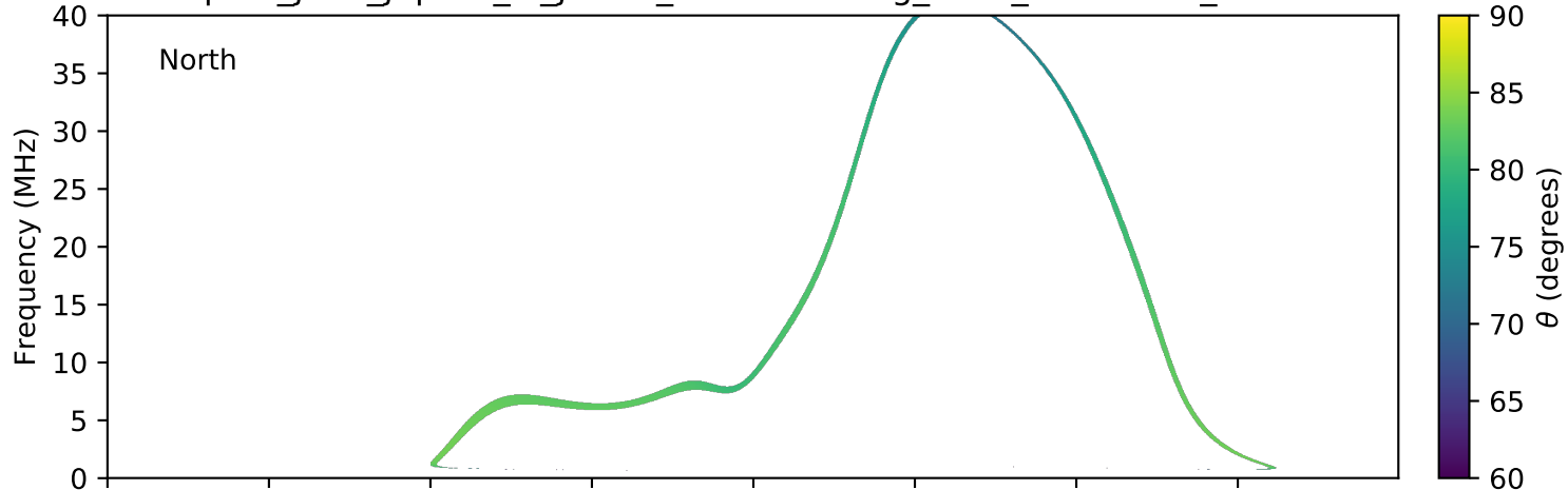
expres_juno_jupiter_io_jrm09_lossc-wid1deg_3kev_20190106_v01.cdf
