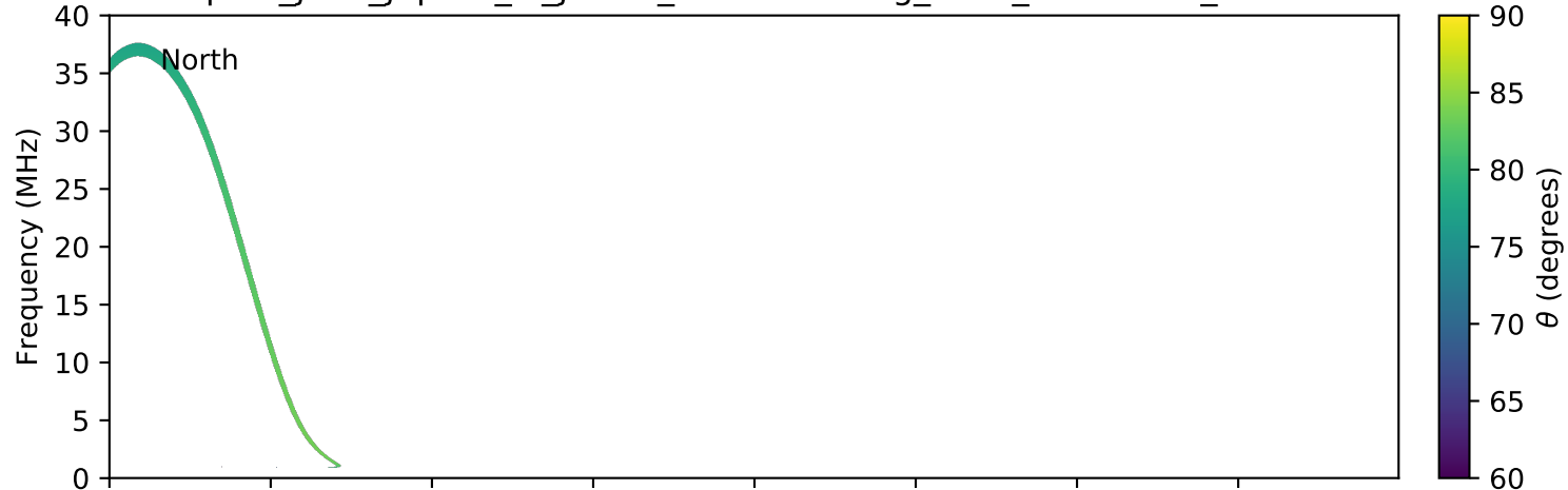
expres_juno_jupiter_io_jrm09_lossc-wid1deg_3kev_20190105_v01.cdf
