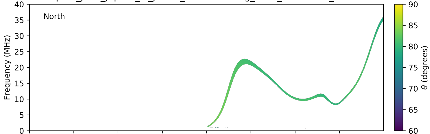
expres_juno_jupiter_io_jrm09_lossc-wid1deg_3kev_20190104_v01.cdf
