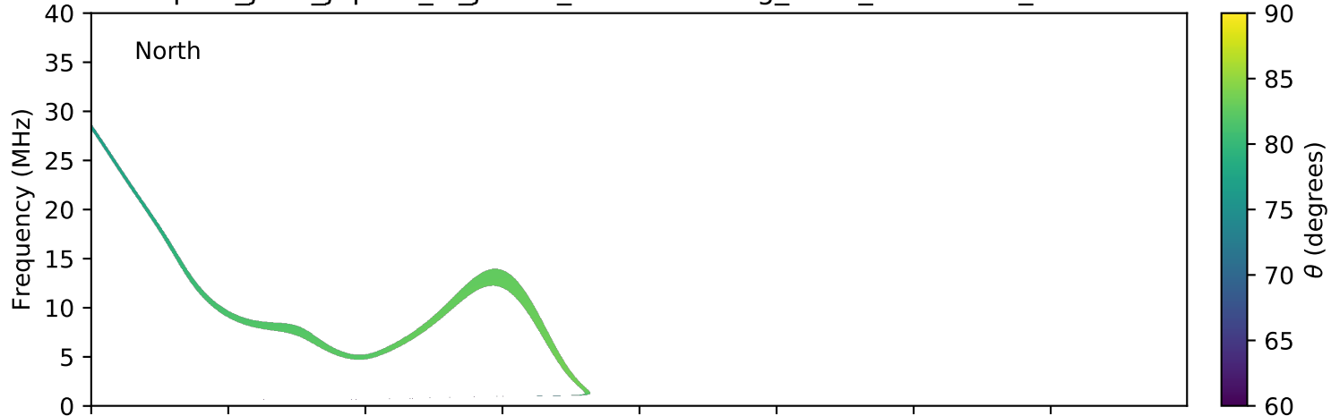
expres_juno_jupiter_io_jrm09_lossc-wid1deg_3kev_20190103_v01.cdf
