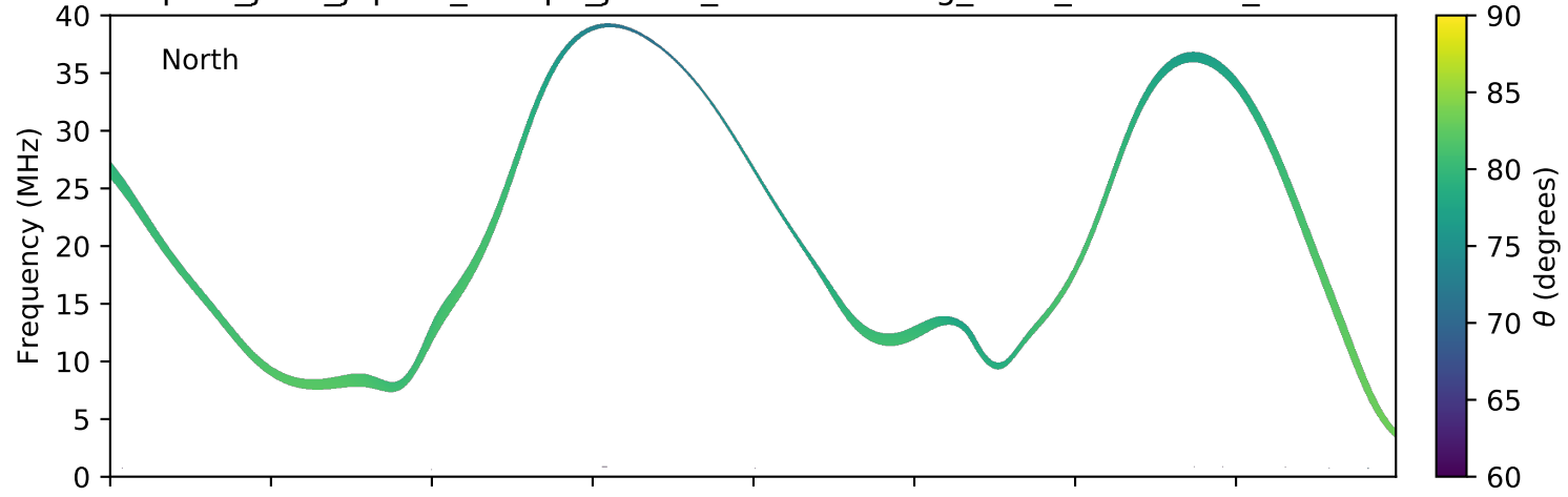
expres_juno_jupiter_europa_jrm09_lossc-wid1deg_3kev_20190129_v01.cdf
