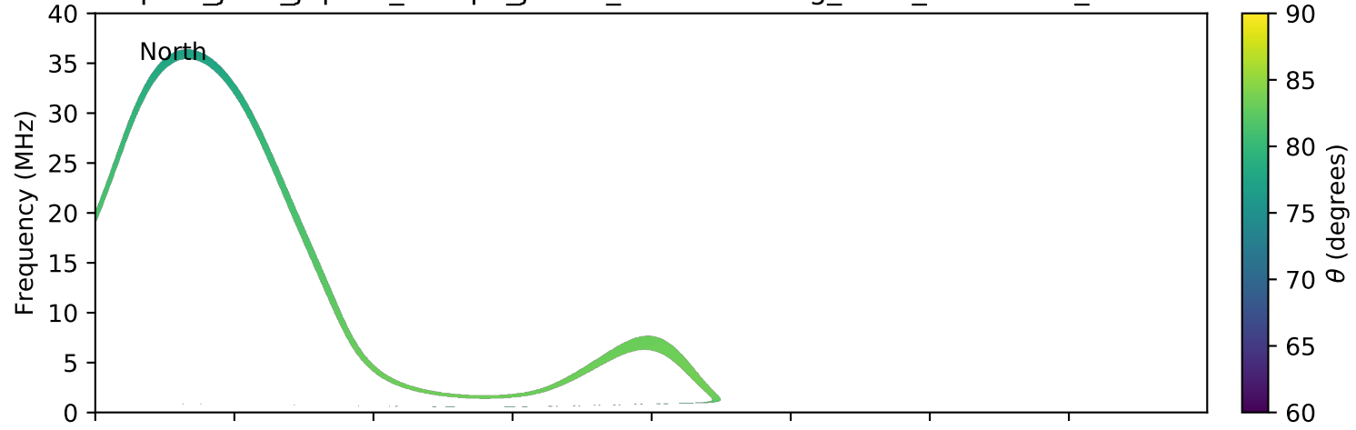
expres_juno_jupiter_europa_jrm09_lossc-wid1deg_3kev_20190119_v01.cdf
