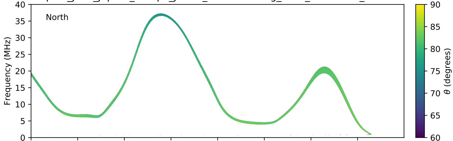
expres_juno_jupiter_europa_jrm09_lossc-wid1deg_3kev_20190115_v01.cdf
