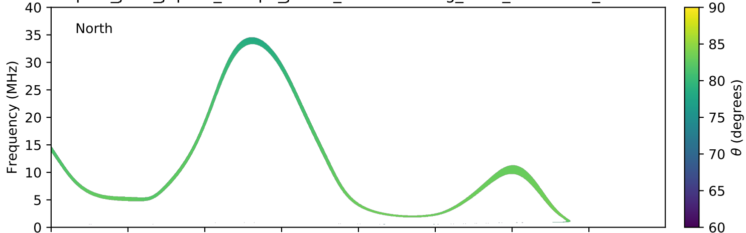
expres_juno_jupiter_europa_jrm09_lossc-wid1deg_3kev_20190108_v01.cdf
