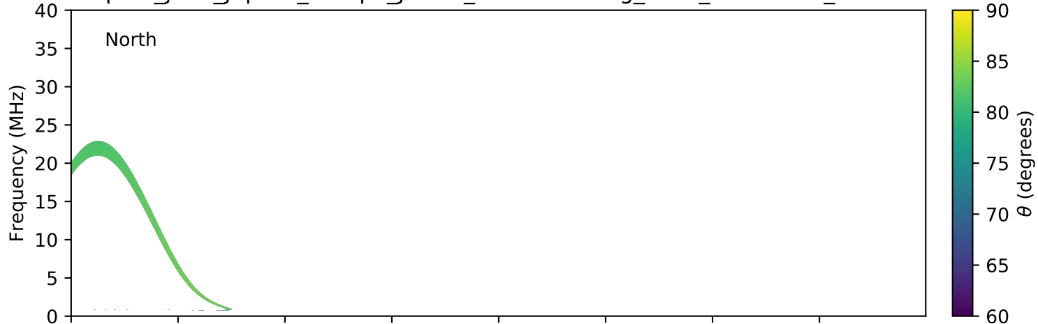
expres_juno_jupiter_europa_jrm09_lossc-wid1deg_3kev_20190105_v01.cdf
