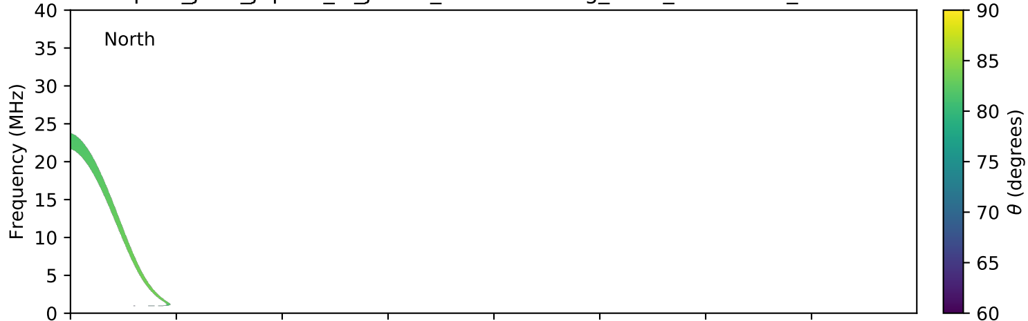
expres_juno_jupiter_io_jrm09_lossc-wid1deg_3kev_20181229_v01.cdf
