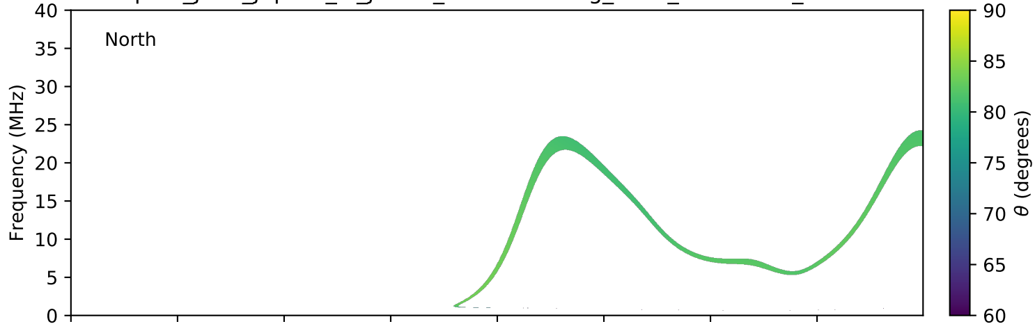
expres_juno_jupiter_io_jrm09_lossc-wid1deg_3kev_20181228_v01.cdf
