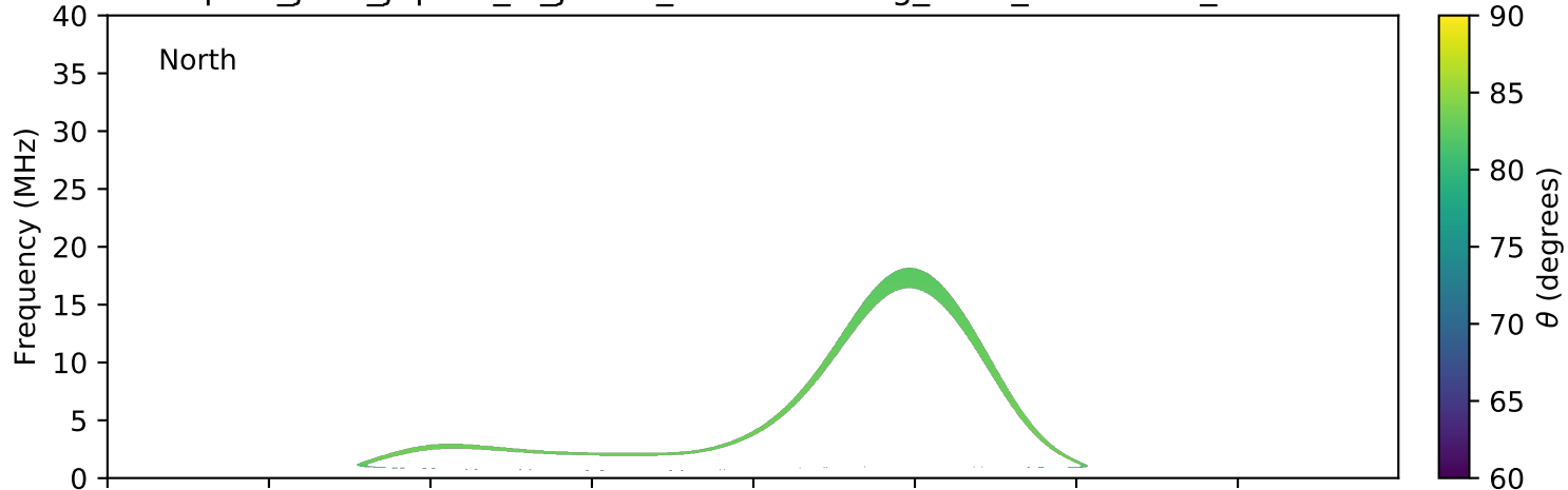
expres_juno_jupiter_io_jrm09_lossc-wid1deg_3kev_20181223_v01.cdf
