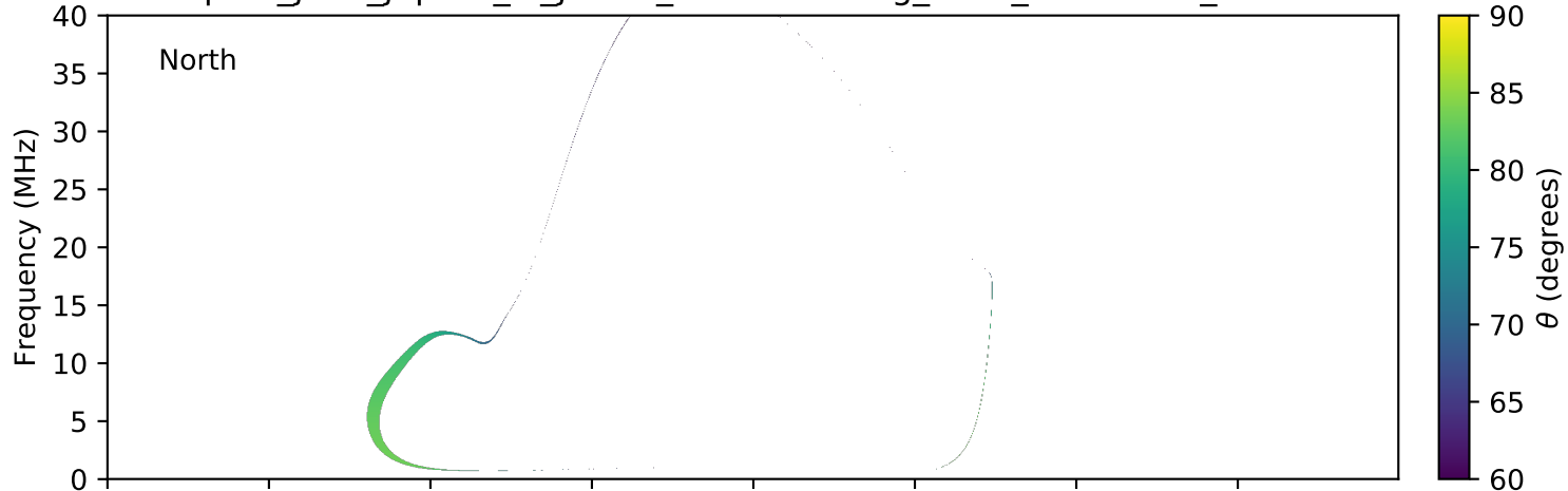
expres_juno_jupiter_io_jrm09_lossc-wid1deg_3kev_20181221_v01.cdf
