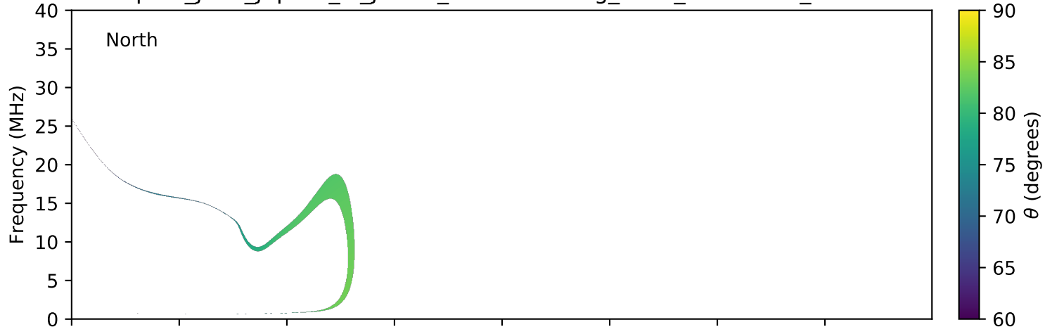
expres_juno_jupiter_io_jrm09_lossc-wid1deg_3kev_20181220_v01.cdf
