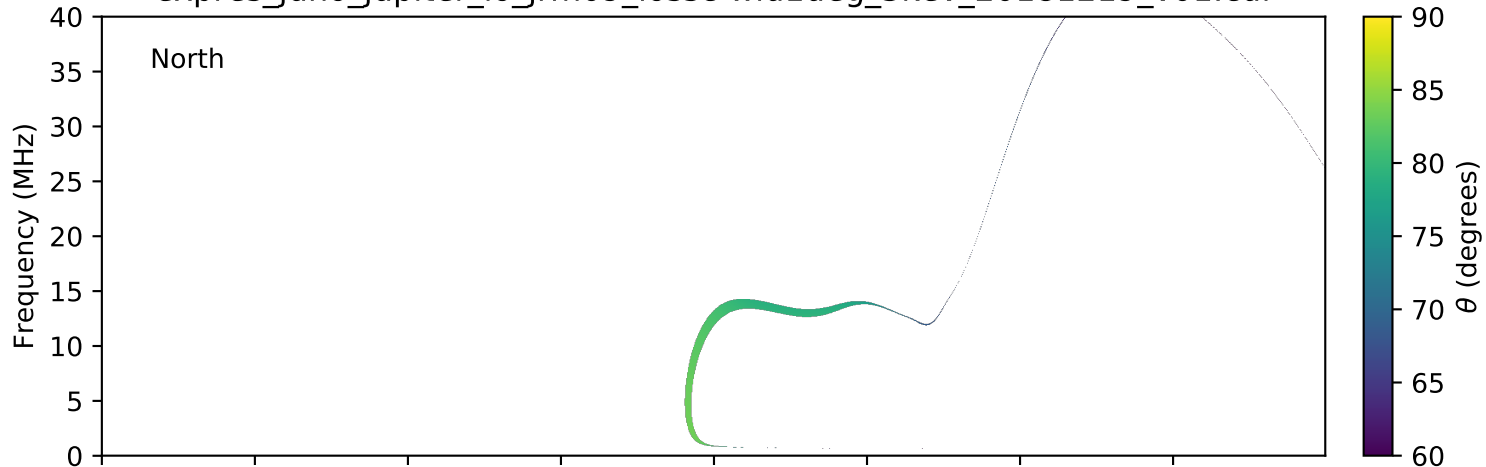
expres_juno_jupiter_io_jrm09_lossc-wid1deg_3kev_20181219_v01.cdf
