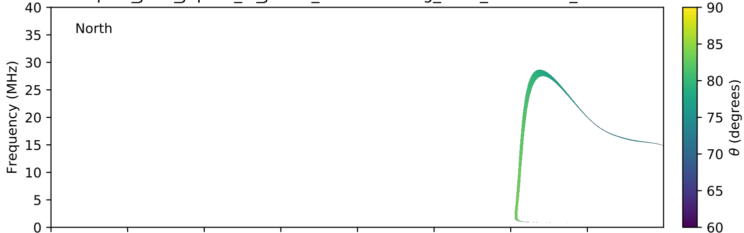
expres_juno_jupiter_io_jrm09_lossc-wid1deg_3kev_20181217_v01.cdf
