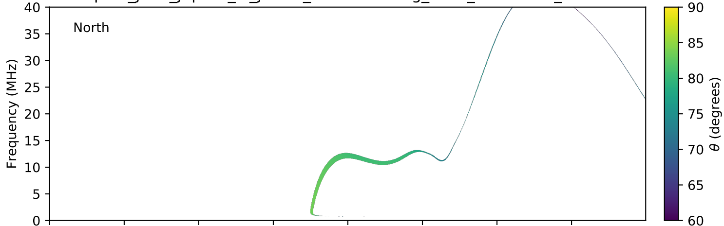
expres_juno_jupiter_io_jrm09_lossc-wid1deg_3kev_20181212_v01.cdf
