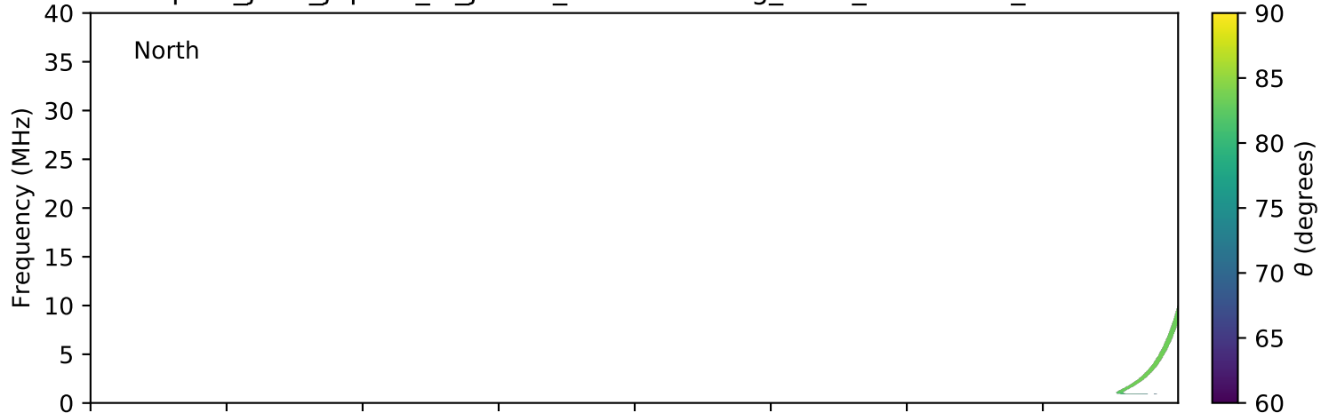
expres_juno_jupiter_io_jrm09_lossc-wid1deg_3kev_20181208_v01.cdf
