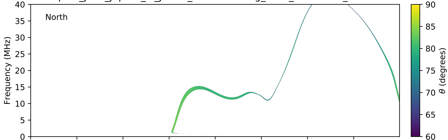
expres_juno_jupiter_io_jrm09_lossc-wid1deg_3kev_20181205_v01.cdf
