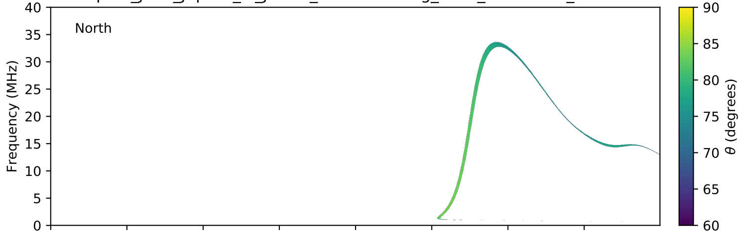
expres_juno_jupiter_io_jrm09_lossc-wid1deg_3kev_20181203_v01.cdf
