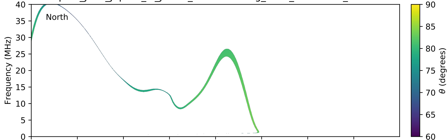
expres_juno_jupiter_io_jrm09_lossc-wid1deg_3kev_20181202_v01.cdf
