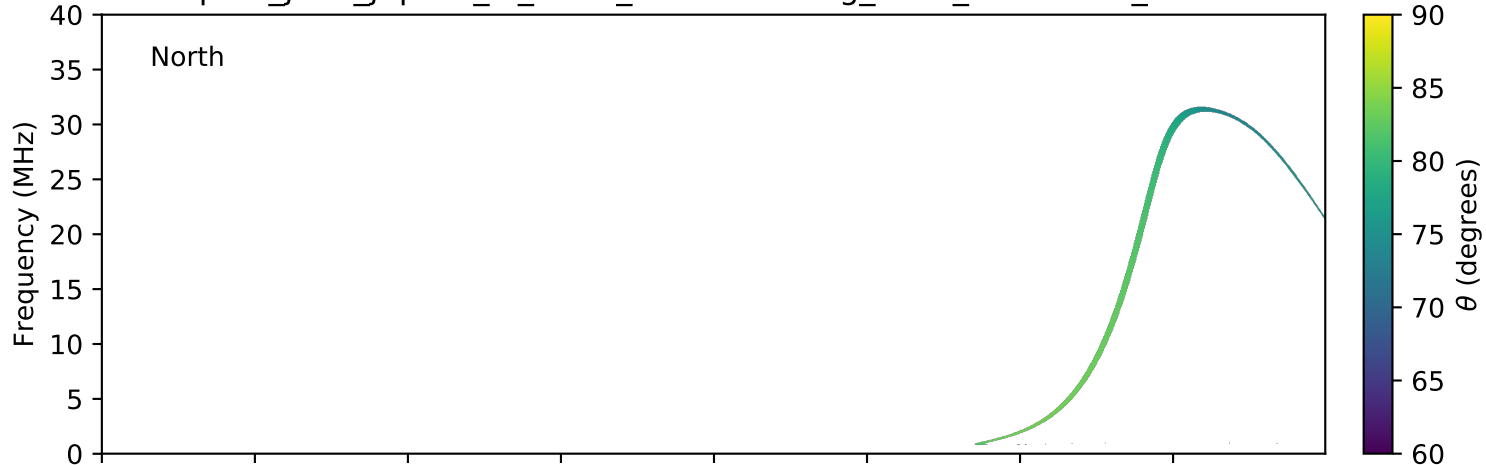
expres_juno_jupiter_io_isaac_lossc-wid1deg_3kev_20181226_v01.cdf
