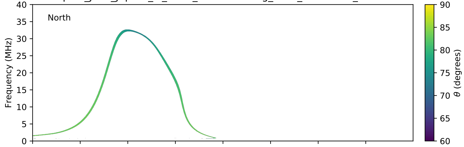
expres_juno_jupiter_io_isaac_lossc-wid1deg_3kev_20181225_v01.cdf
