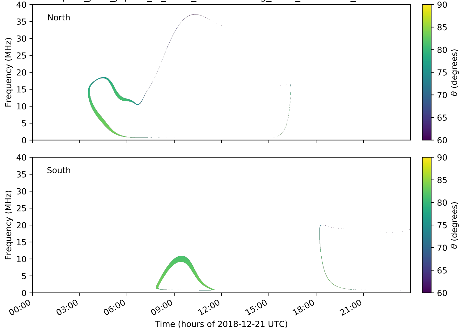
expres_juno_jupiter_io_isaac_lossc-wid1deg_3kev_20181221_v01.cdf
